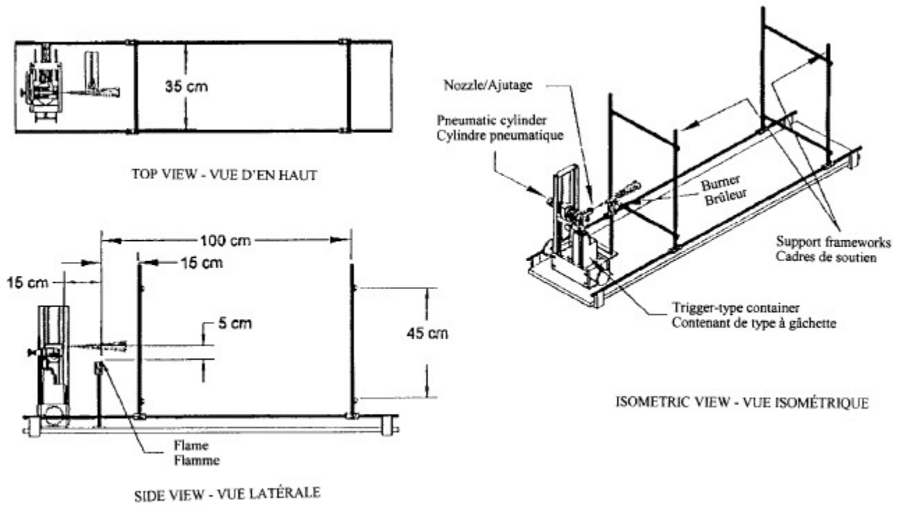
FIGURE 3 Holding Apparatus for a Trigger-Type Container Isometric View
